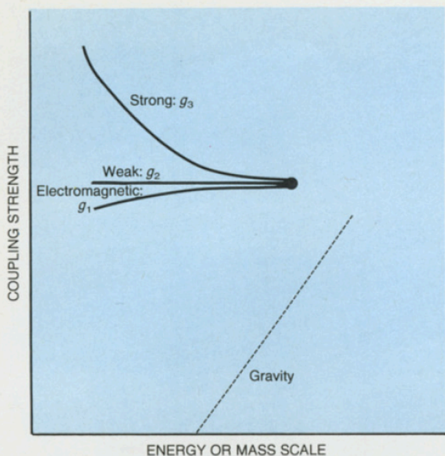
The running of the strong, weak and electromagnetic couplings, extrapolated to very high mass scales, can result in their meeting at a point. This occurs if these three interactions, as observed at low energy, all result from the spontaneous breakdown of a unified theory at a large mass scale. The gravitational coupling, shown schematically on this plot, starts out very much smaller than the other couplings but would join them if extrapolated to about 10^{19} GeV. Figure 6
